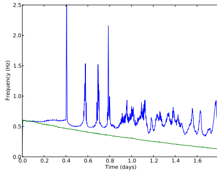
Fig. 2: E activity during pruning with (blue / upper) and without (green / lower) compensatory synaptic scaling. Run time 160,000 s ( \approx 44 h).
